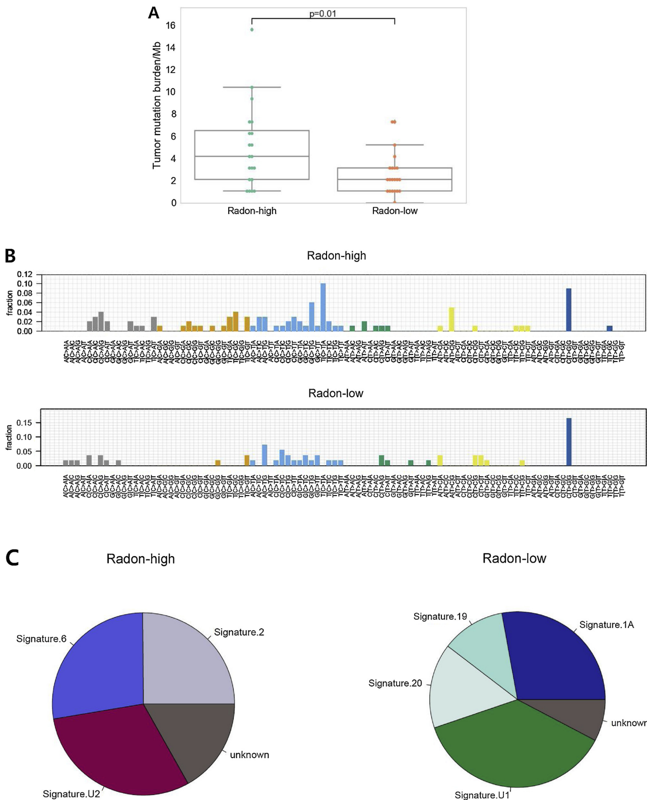
Fig. 2. A. Median tumor mutation burden (TMB) of radon-high group was 4.94 vs. 2.62 mutations/Mb in radon-low group ( P = 0.01 ). B. Comparison of mutation signatures between radon-high vs. radon-low groups. There were six classes of base substitution – C > A, C > G, C > T, T > A, T > C, and T > G, and we incorporated information on the bases located immediately 5' to 3' to each mutated base to obtain 96 possible mutations. C. Proportions of selected mutational signatures in radon-high and radon-low groups.
